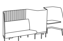
Lite Settee + Double Workpod 纤致沙发+双人工作站 W3515 D743 H1600
