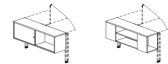
Single Sliding Cabinet 单趟门柜 W: 1200,1400,1600 D: 360 Three Sides Open Cabinet 三面开口柜 W: 1200,1400,1600 H: 360
