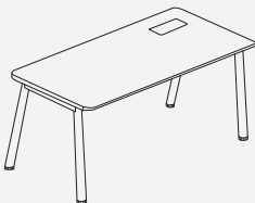
Straight Desk with Round Leg 直形台带圆柱台脚 W : 1400, 1500, 1600, 1800 D : 700, 800 H : 750
