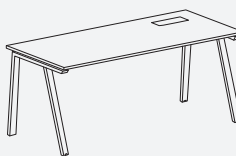
Straight Desk with Trapezoid Leg 直形台带梯形台脚 W : 1400, 1500, 1600, 1800 D : 700, 800 H : 750
