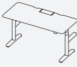
Height-adjustable Single Bench 单边升降共享台 W:1400,1500,1600,1800 D: 600,700,800 H: 650-1250
