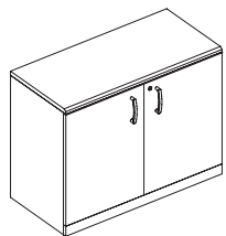
Low cabinet, wooden doors MYC0710W ( ) - W1000 x D470 x H760
