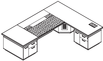
Executive desk w/ pedestal, extension, w/o LCD lifter MY2422P(L/R)(C/H) ( ) - W2400 x D2200 x H760 MY2824P(L/R)(C/H) ( ) - W2800 x D2400 x H760 MY3024P(L/R)(C/H) ( ) - W3000 x D2400 x H760 MY3226P(L/R)(C/H) ( ) - W3200 x D2600 x H760 MY3426P(L/R)(C/H) ( ) - W3400 x D2600 x H760 MY3628P(L/R)(C/H) ( ) - W3600 x D2800 x H760 MY3828P(L/R)(C/H) ( ) - W3800 x D2800 x H760
