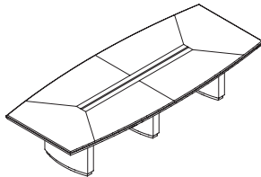
Boat-shaped conference table MYCB2412(C/H) ( ) - W2400 x D1200 x H760 MYCB2812(C/H) ( ) - W2800 x D1200 x H760 MYCB3214(C/H) ( ) - W3200 x D1400 x H760 MYCB3615(C/H) ( ) - W3600 x D1500 x H760 MYCB3815(C/H) ( ) - W3800 x D1500 x H760 MYCB4018(C/H) ( ) - W4000 x D1800 x H760
