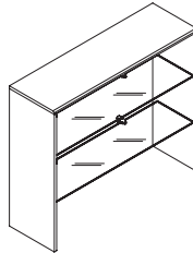
Credenza, w/ glass shelves MYC1215 ( ) - W1500 x D470 x H1270
