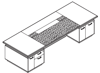
Executive desk w/ pedestal, w/o extension MY2811P(L/R)(C/H) ( ) - W2800 x D1150 x H760 MY3011P(L/R)(C/H) ( ) - W3000 x D1150 x H760 MY3211P(L/R)(C/H) ( ) - W3200 x D1150 x H760
