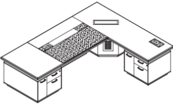
Executive desk w/ pedestal, extension & LCD lifter MY2824LP(L/R)(C/H) ( ) - W2800 x D2400 x H760 MY3024LP(L/R)(C/H) ( ) - W3000 x D2400 x H760 MY3226LP(L/R)(C/H) ( ) - W3200 x D2600 x H760 MY3426LP(L/R)(C/H) ( ) - W3400 x D2600 x H760 MY3628LP(L/R)(C/H) ( ) - W3600 x D2800 x H760 MY3828LP(L/R)(C/H) ( ) - W3800 x D2800 x H760
