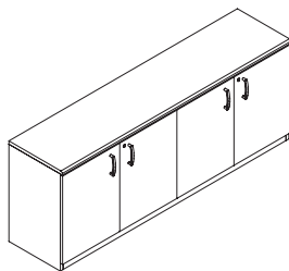
Low cabinet, wooden / glass doors MYC0720W ( ) - W2000 x D470 x H760 MYC0720G ( ) - W2000 x D470 x H760
