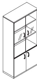
High cabinet, wooden doors & glass doors MYC2010G ( ) - W1000 x D470 x H2030
