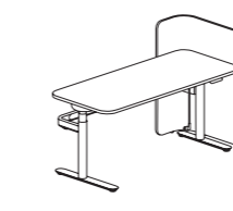
Side Straight Screen (L/R) 侧边直形屏风 (左/右) W: 1200 D: 1100,1200
