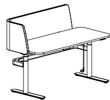
L Long Wave Screen (L&R) L型长弧屏风 (左/右) W: 1400,1500,1600,1800 D: 1100,1200
